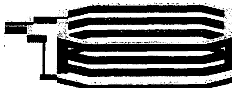
Figure 2. The primary of the toroidal transformer balun. Note the via for interconnection between metal layers.
