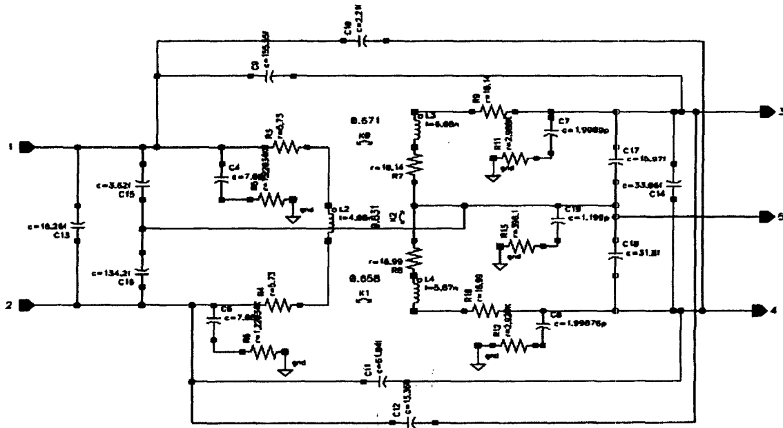
Figure 4. Five-port transformer balun circuit model.
